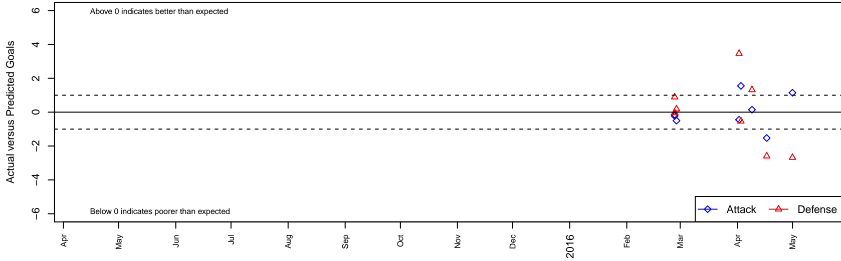
Quad City Fusion G97 Dots are actual minus expected GF (blue circles) and GA (red triangles). Blue line is smoothed change in attack strength. Red is smoothed change in defense strength.
